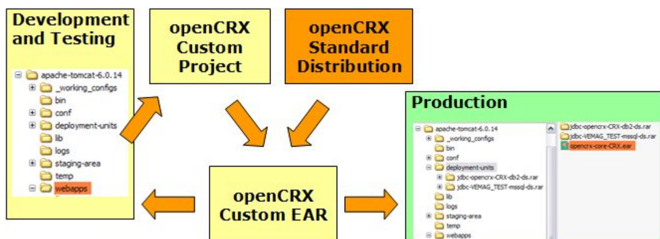
Figure 5: openCRX Development and Customizing with Custom Project
