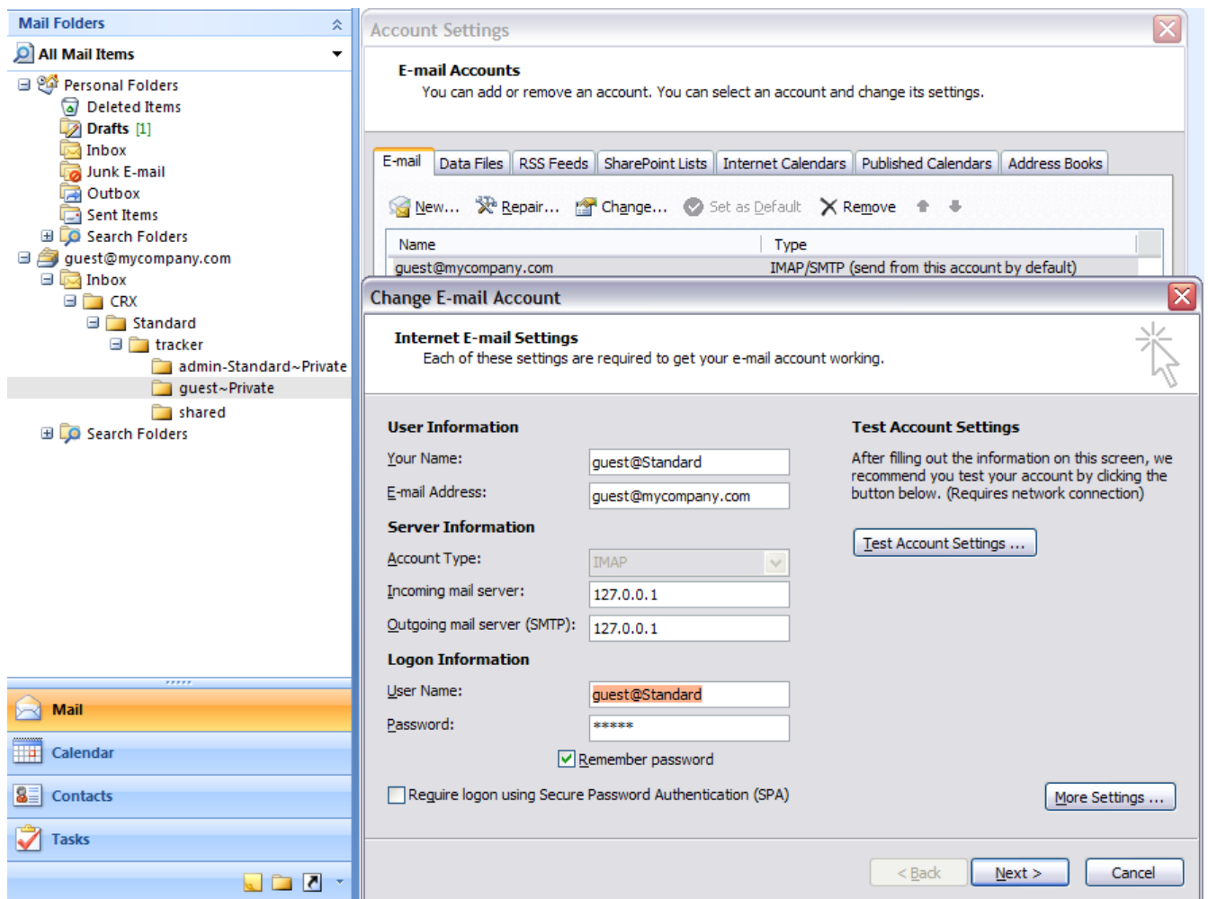
Figure 64: MS Outlook IMAP Configuration
