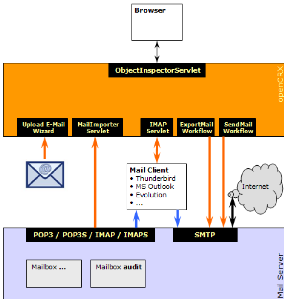
Figure 37: Flow of e-mail messages between openCRX, MTA and MUA
