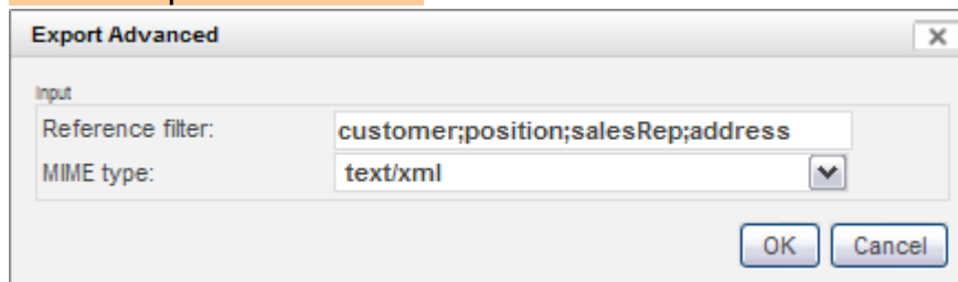
Figure 73: Exporting SalesOrder as XML File
