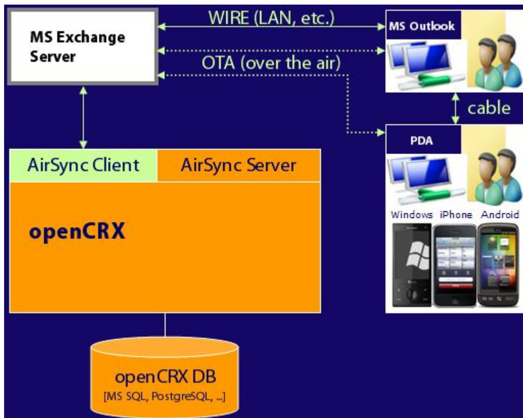
Figure 66: openCRX AirSync Client – backend-sync with Exchange
