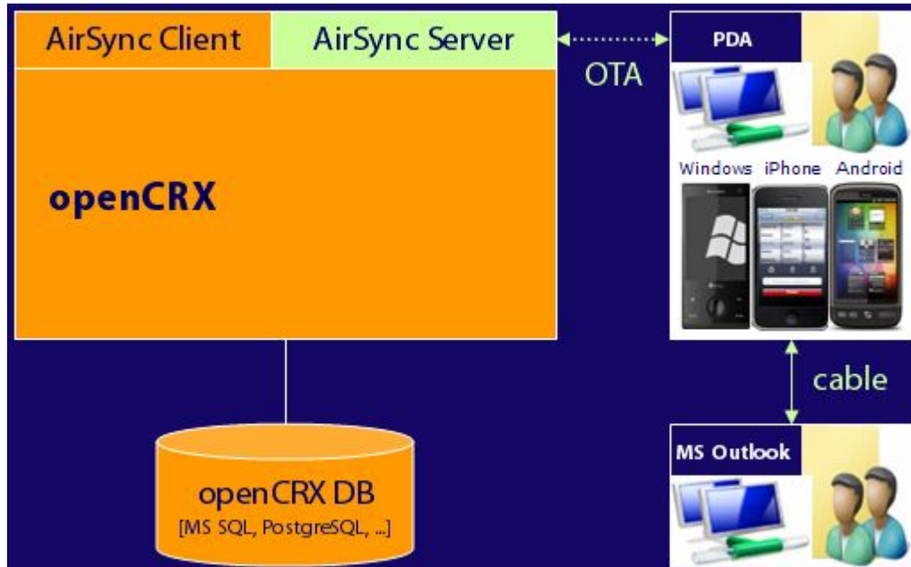
Figure 65: openCRX AirSync Server – Over The Air (OTA) Synchronization
